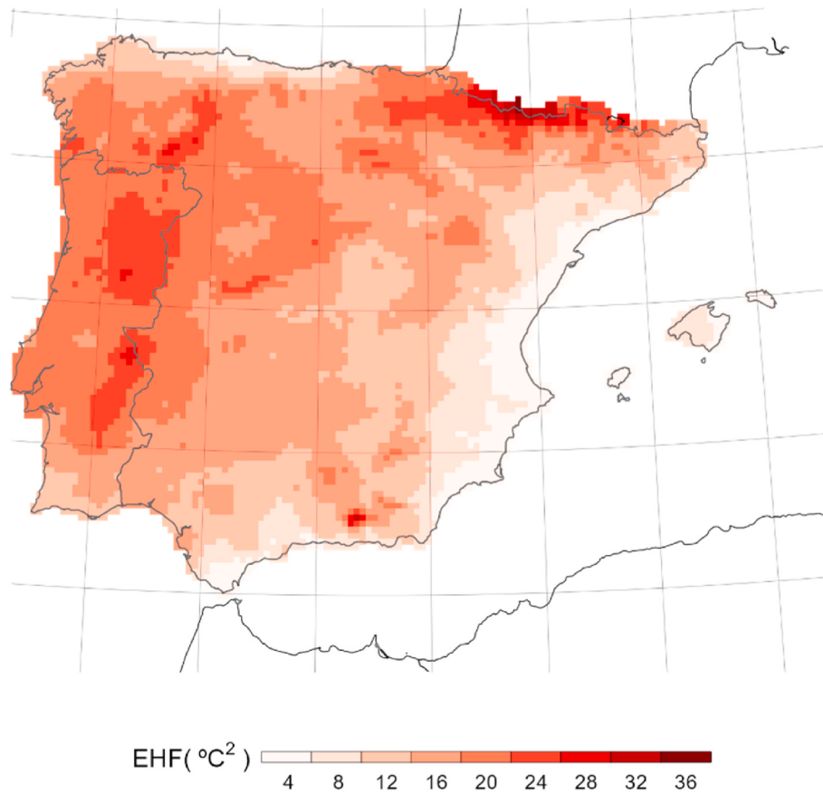
Fig. 4. The 95th percentile of positive EHF values for the period 1950–2020.
