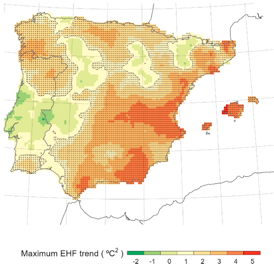
Fig. 7. Trend of the maximum of EHF for the period 1950–2020. Values are expressed in °C 2 /decade.
