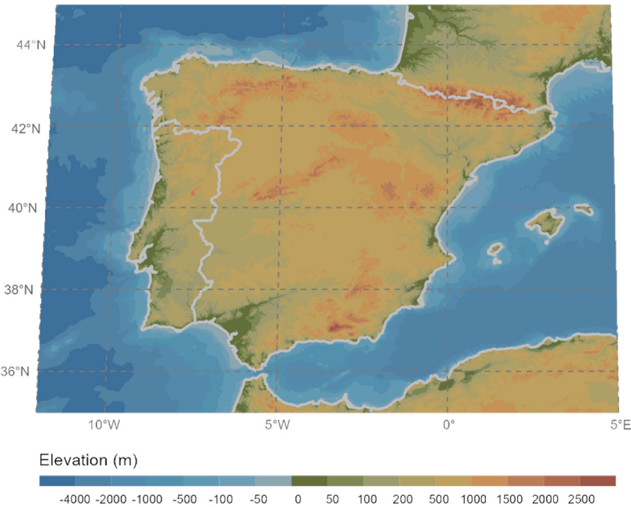
Fig. 1. Study area showing the limits of the IP and terrain elevation.
