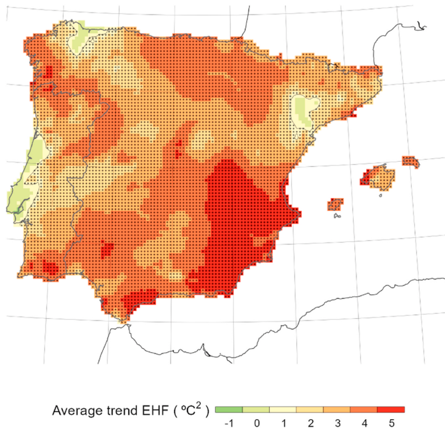
Fig. 6. Average trend in the intensity of events with positive EHF for the period 1950–2020. Values are expressed in ^{\circ}\text{C}^2/\text{decade} .
