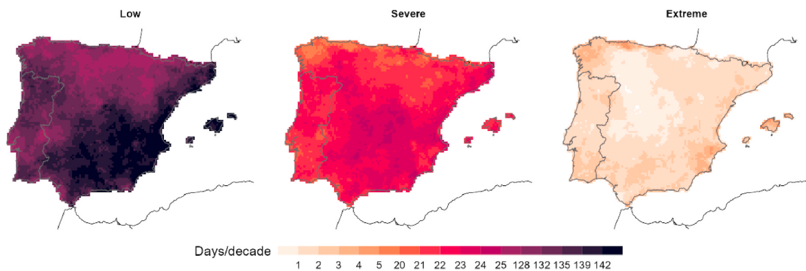
Fig. 5. Average duration of severity levels in days/decade for the period 1950–2020.
