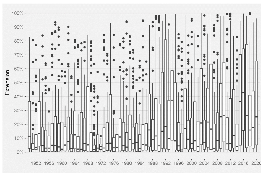
Fig. 9. Distribution of the spatial extensions of heat waves by year in the IPB (1950–2020).
