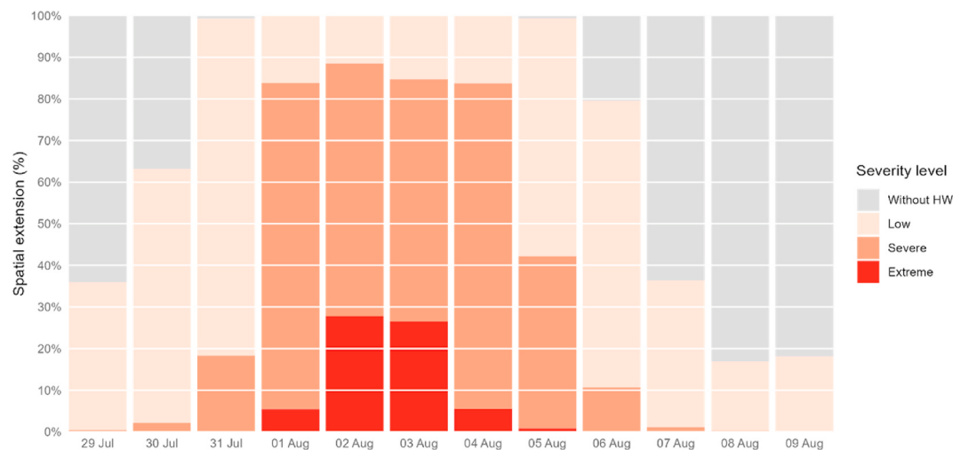
Fig. 13. Spatial extension of the heat wave for the period 2018-07-29 to 2018-08-09.
