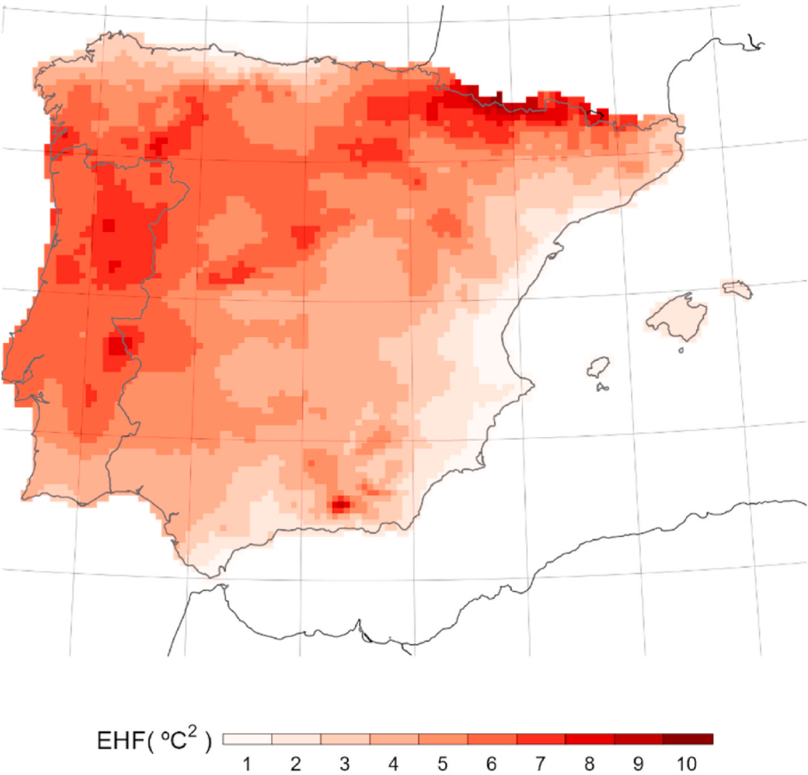
Fig. 2. Average positive EHF values for the period 1950–2020.
