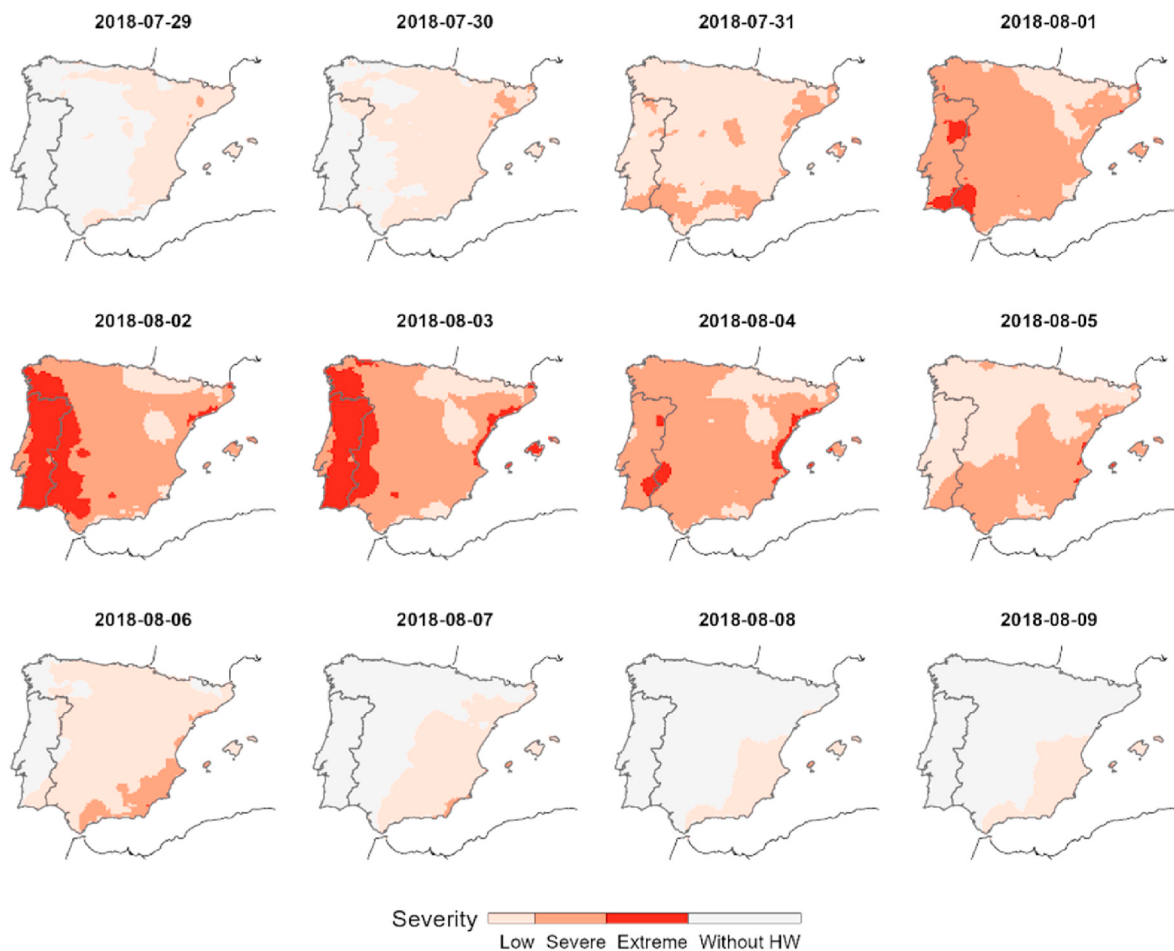
Fig. 12. Severity threshold for the period 2018-07-29 to 2018-08-09 (in °C 2 ).
