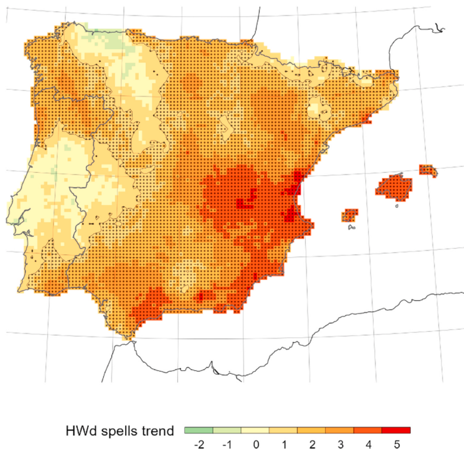
Fig. 8. Trend in heat wave spells in days (HWD) for the period 1950–2020. Values are expressed in days/decade.
