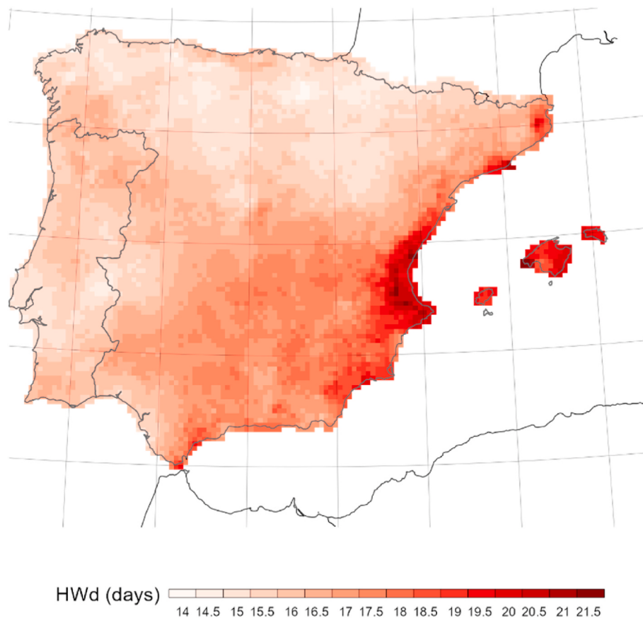
Fig. 3. Annual average heat wave days (HWD) for the period 1950–2020.
