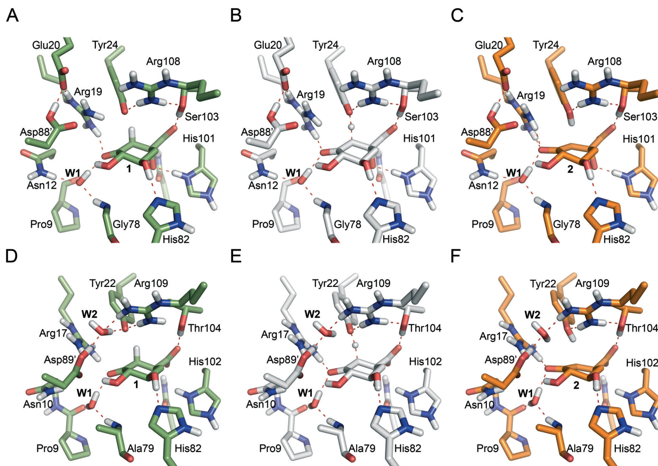
Fig. 5 Representative geometries of the catalytic tyrosinate (A & D), TS1 (B & E) and enolate intermediate 2 (C & F) for the 2 nd step of the MtDHQ2 (A–C) and HpDHQ2 (D–F) mechanism. Geometries were taken from the potential energy surface. Relevant residues and water molecules are shown and labeled. Key hydrogen bonding interactions and bonds broken/formed are indicated as red dashed lines.
