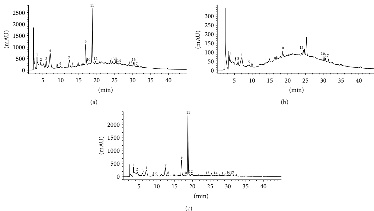
FIGURE 2: Chromatograms acquired at 280 nm by HPLC-DAD-UV. (a) Chromatogram of the crude extract without fractionation process. (b) Chromatogram of the residue of the crude extract that remains in the extraction cell after the fractionation process ( E_{Cell} ). (c) Chromatogram of the fraction obtained under optimal conditions ( E_{140} ).
