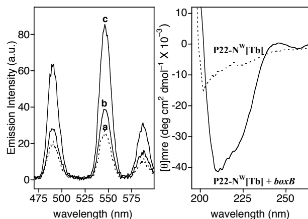
Figure 3. Left: a) Time-resolved luminescence emission (0.2 ms delay time) of a 100 nM solution of P22-N W [Tb] in 10 mM HEPES buffer, 100 mM NaCl, pH 7.6; b) in the presence of 300 ng/mL total protein cell lysate; c) after addition of 1 eq. of boxB RNA. Right: Circular dichroism of a 5 \mu\text{M} solution of the peptide P22-N W [Tb] sensor in 10 mM phosphate buffer, 100 mM NaCl, pH 7.5 (dashed line), and in the presence of 1 equiv. of boxB RNA (solid line).
