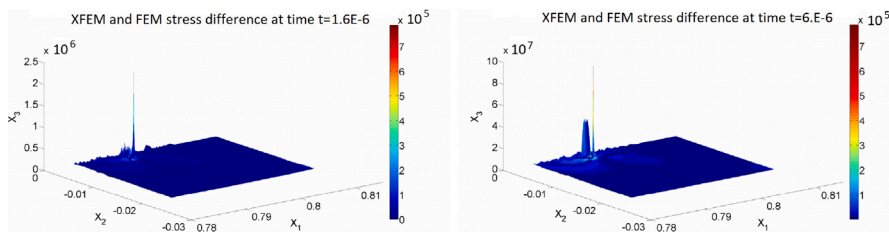
Fig. 10. Difference between Von Mises norm for stress computed with XFEM and FEM at time t = 1.6\text{E}-6 s and t = 6.\text{E}-6 s.
