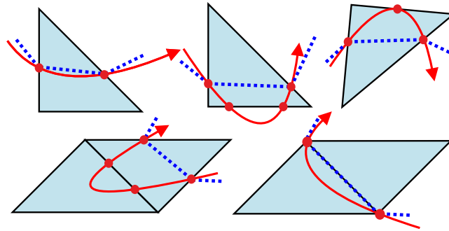
Fig. 5. Linear approximation of the interface within each element.
