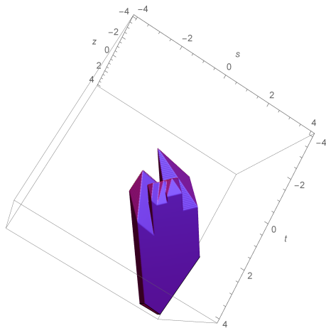
Figure 4.6.3: \mathfrak{K}
