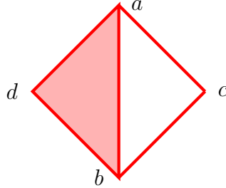
Figura 2.5: Collapse but not edge collapse.
