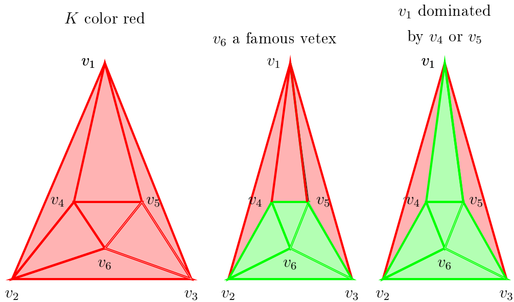
Figura 2.3: Strong collapse algorithm, part 1.
