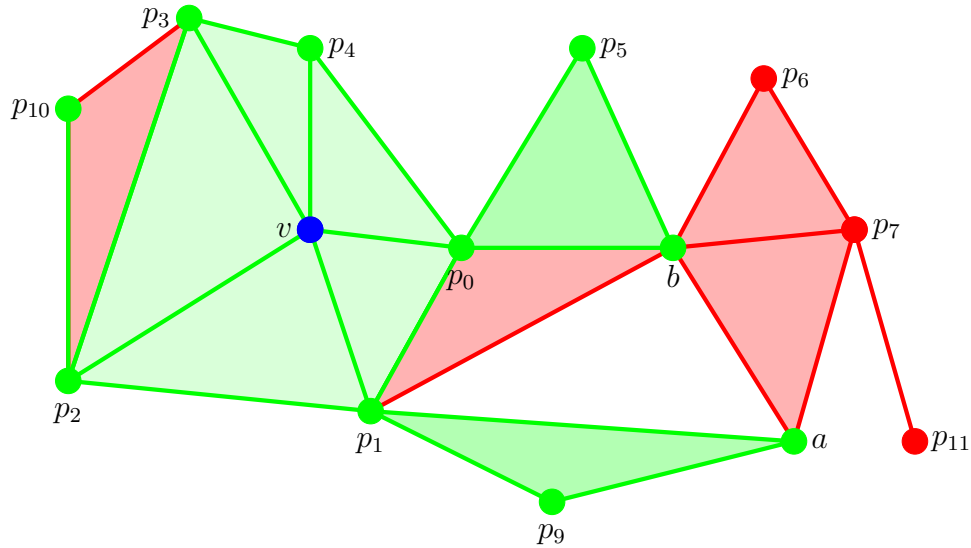
Figura 2.9: Edge collapse algorithm, part 3.
