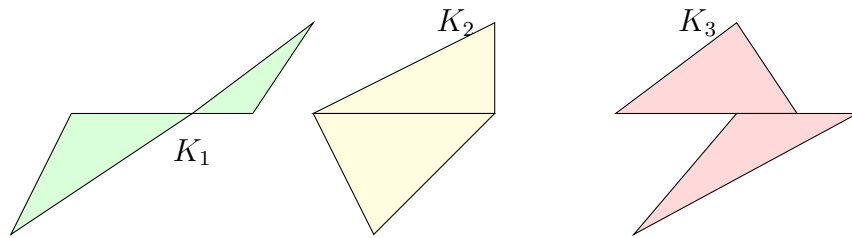
Figura 1.1: Simplicial complex.
