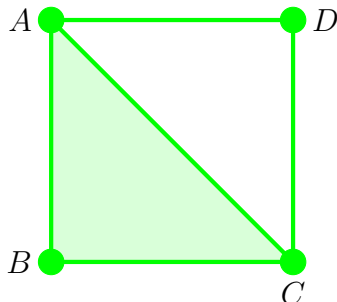
Figura 1.2: Geometric realization of a simplicial complex
