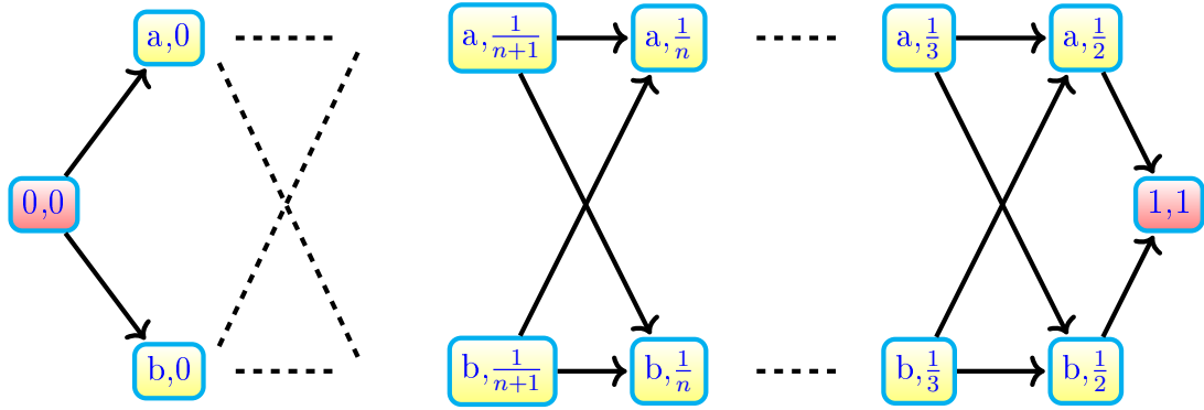
Figura 4.3: P -collapsible, but not B^+ -collapsible space.
