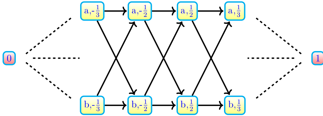
Figura 4.5: P -collapsible space with no elementary B^+ -collapse
