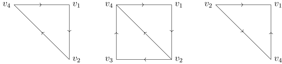
Figura 5.4: Cyclic graph with a dominated vertex.
