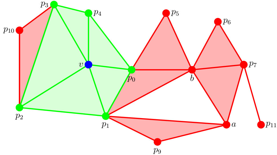
Figura 2.8: Edge collapse algorithm, part 2.
