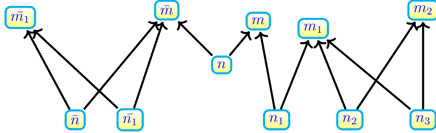
Figura 4.7: \mathcal{B} -core and \mathcal{P} -core space
