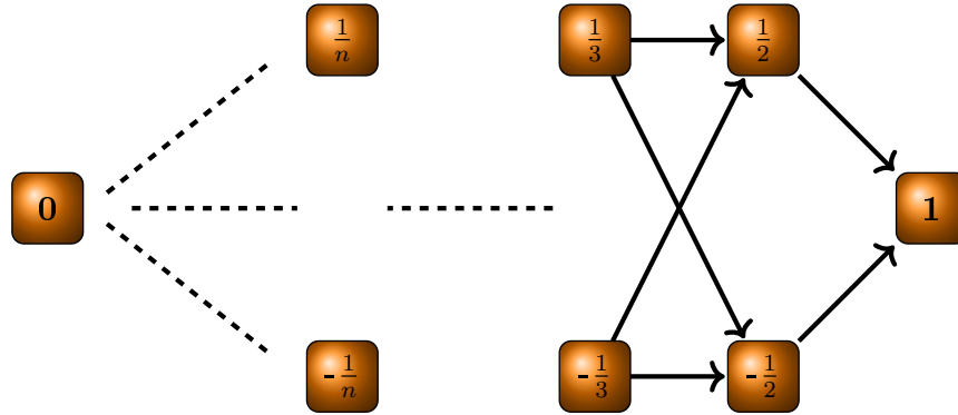
Figura 4.4: P -collapsible and B^+ -collapsible space.
