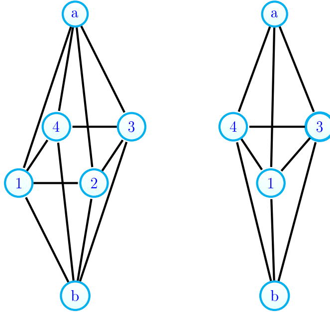
Figura 3.1: Simplicial complex (matroid) can be edge collapsed but not collapse nor strong collapse.
