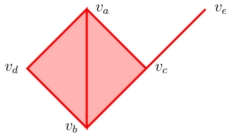
Figura 4.9: The associated simplicial complex \mathcal{K}(X) .
