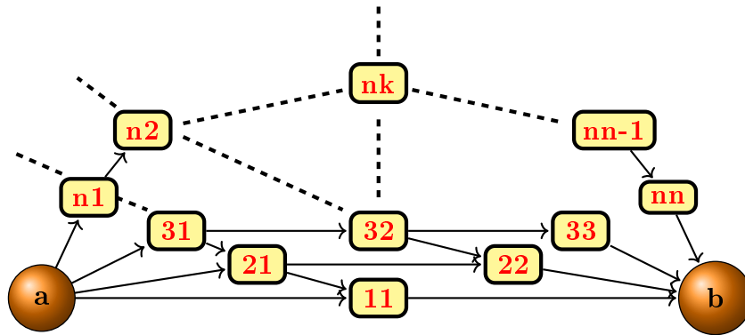
Figura 4.2: Infinite space which is a finite-chain space
