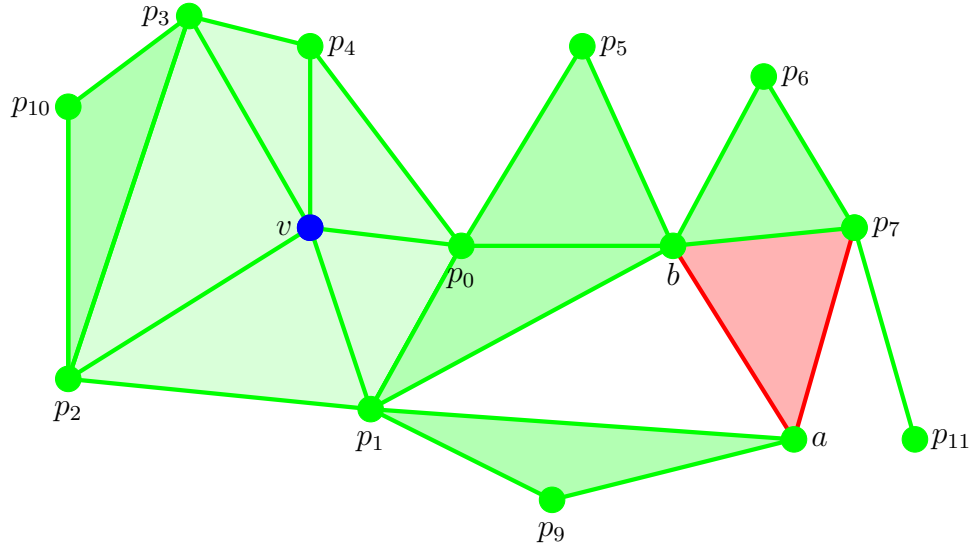
Figura 2.11: Edge collapse algorithm, part 5.
