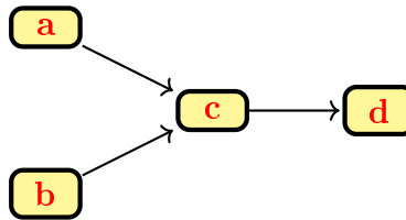
Figura 4.1: Hasse diagram
