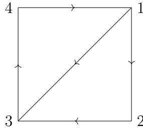
Figura 5.2: Cyclic graph includes a +ve and -ve dominated vertex.
