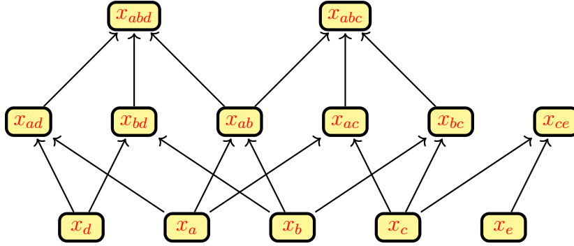
Figura 4.10: The associated finite space \mathcal{X}(\mathcal{K}(X)) .
