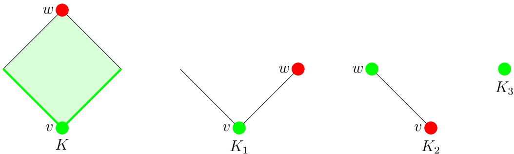
Figura 2.2: Strong collapse a simplicial complex
