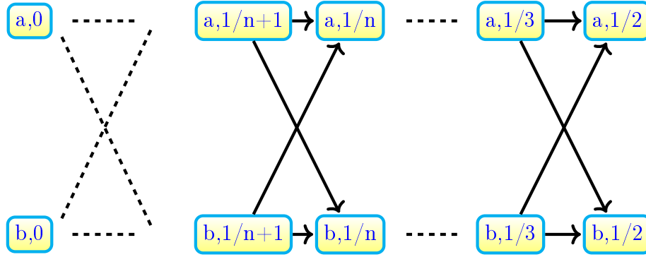
Figura 4.6: Finite bounded but not fp-space.
