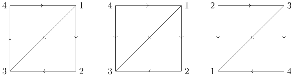
Figura 5.1: Cyclic and not cyclic graphs
