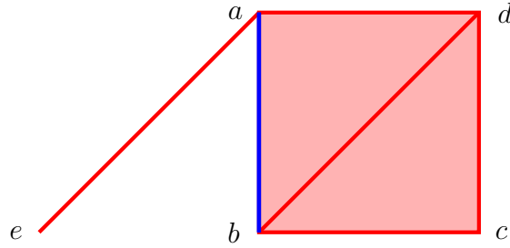
Figura 2.6: Edge collapse but not strong collapse.
