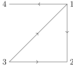
Figura 5.3: Not cyclic graph.
