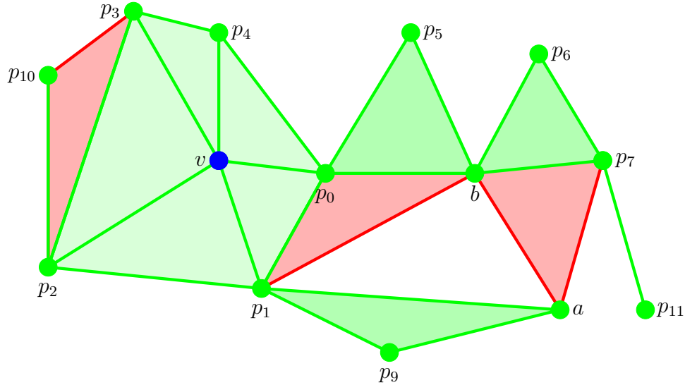
Figura 2.10: Edge collapse algorithm, part 4.
