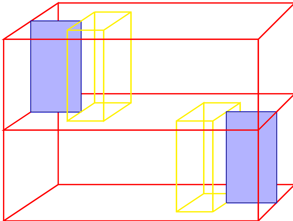
Figura 1.4: Bing's house with two rooms.
