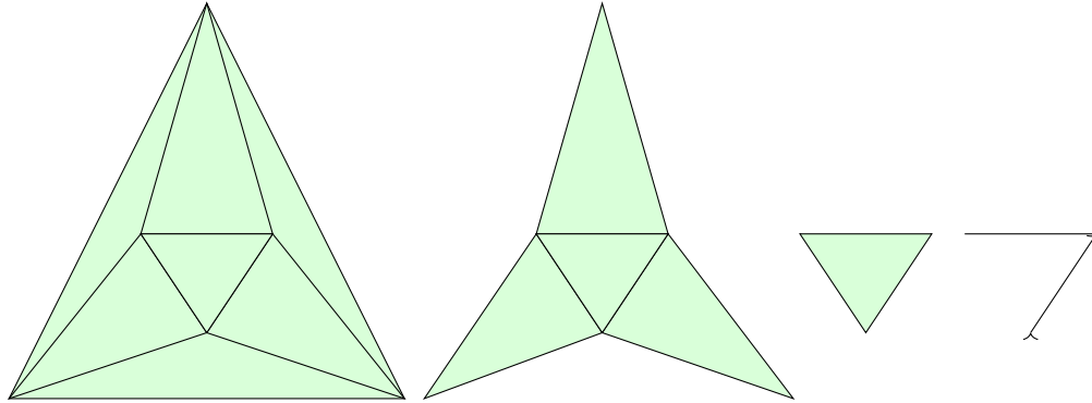
Figura 2.1: Collapse a simplicial complex
