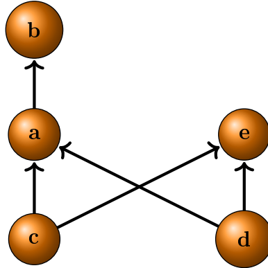
Figura 4.8: Finite Alexandroff space X .
