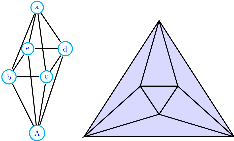
Figura 1.3: Simplicial complex.
