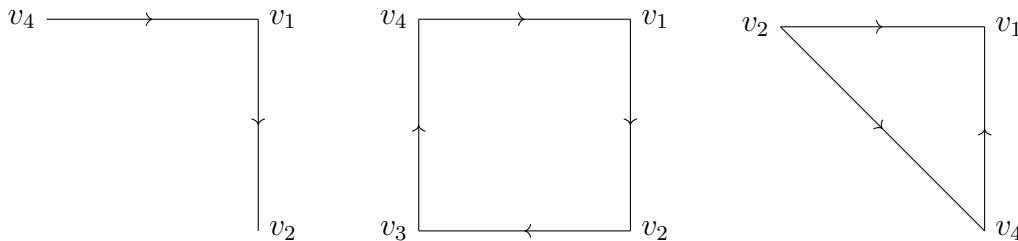
Figura 5.5: Cyclic graph without dominated vertices.
