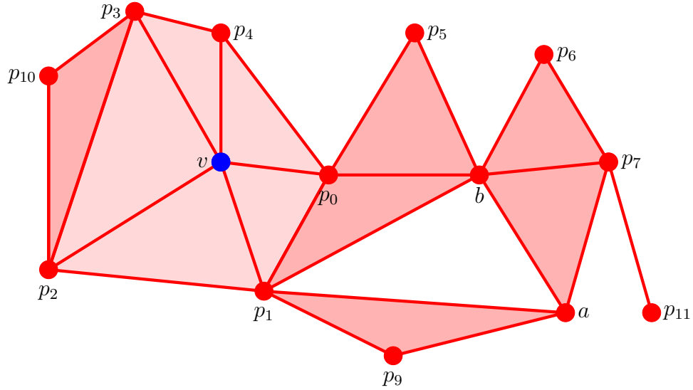
Figura 2.7: Edge collapse algorithm, part 1.
