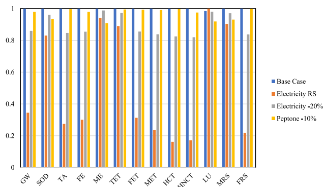
Fig. 8. Sensitivity assessment of the environmental profile of GM valorization for resveratrol production considering a reduction on the use of electricity by 20%, the use of renewable resources for electricity production and on peptone dose of 10%.
