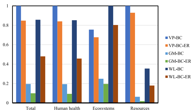
Fig. 11. Comparison of the environmental loads of the assessed scenarios using the ReCiPe EndPoint methodology.
