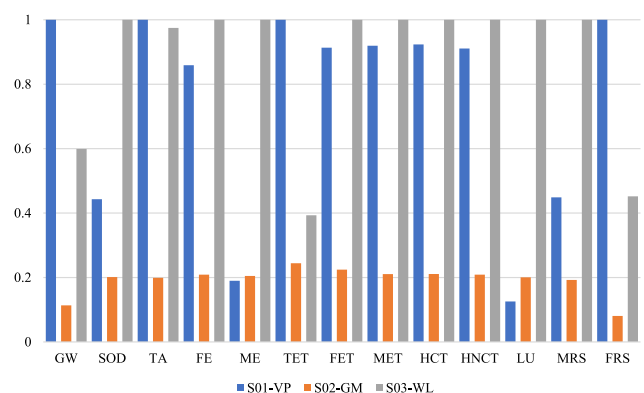
Fig. 10. Comparison of the environmental loads of the assessed scenarios using the ReCiPe MidPoint methodology.
