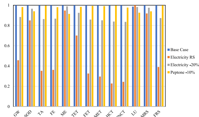
Fig. 9. Sensitivity assessment of the environmental profile of GM valorization for resveratrol production considering a reduction on the use of electricity by 20%, the use of renewable resources for electricity production and on peptone dose of 10%.
