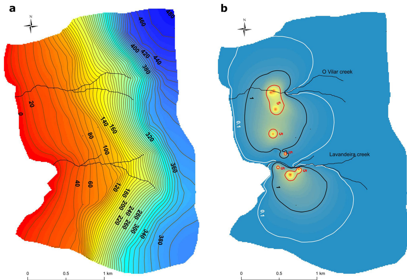
Fig. 7 Contour lines of the a computed steady-state hydraulic heads (lines every 10 m) and b computed drawdown ( s ) during the dry season for the maximum pumping rates in wells 1–8. White, black and red lines
