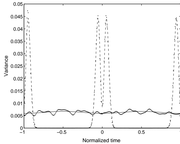
Figure 2.12: Input variance in two unit intervals obtained from Eq. (2.50) (dashed curve) and through a numerical estimate over 100 sample trains (dots); output variance for \gamma/\alpha = 1/4 in two unit intervals obtained from Eq. (2.51) (solid line) and through a numerical estimation (dots). Parameters as in Fig 2.11.
