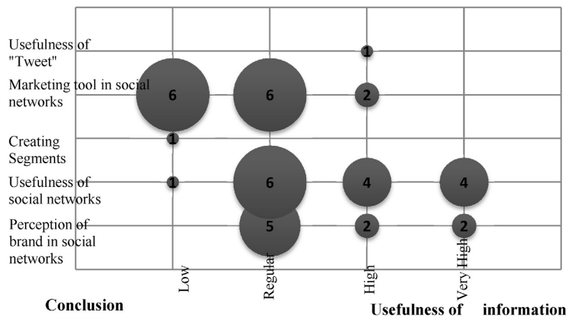
Fig. 5. Global systematic mapping 2014–2015.
