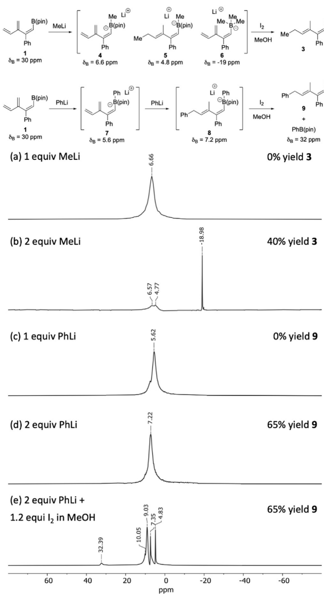
Figure 1. Mechanism investigation and reaction optimization via 11 B NMR analysis.
