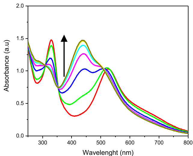
Fig. 3. Time evolution of DPPH (1.125 × 10 -4 M) spectra after adding Ag 5 (≈3.7 × 10 -7 M). Spectra were taken every 2 min.
