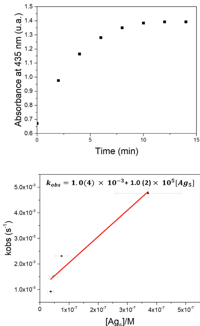
Fig. 4. a) Evolution of the maximum at 435 nm, ascribed to DPPH - anion, for DPPH - 1.12 \times 10^{-4} M in the presence of \approx 3.7 \times 10^{-7} M Ag_5 in 3:1 (v/v) methanol:water solution. b) Kinetic constant versus [Ag_5] in the range 20–200 \mu g/L ( \sim 3.7 \times 10^{-8} M – \sim 3.7 \times 10^{-7} M) with a constant DPPH - concentration of 1.12 \times 10^{-4} M in methanol.
