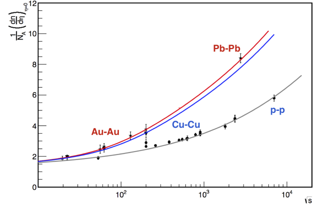
FIGURE 7. Comparison of the evolution of the mid-rapidity multiplicity with energy from the CSPM and data for p+p and A-A collisions. Lines are from the model for p+p (gray), Cu-Cu (blue) and red lines for Au-Au/Pb-Pb [85-89].
