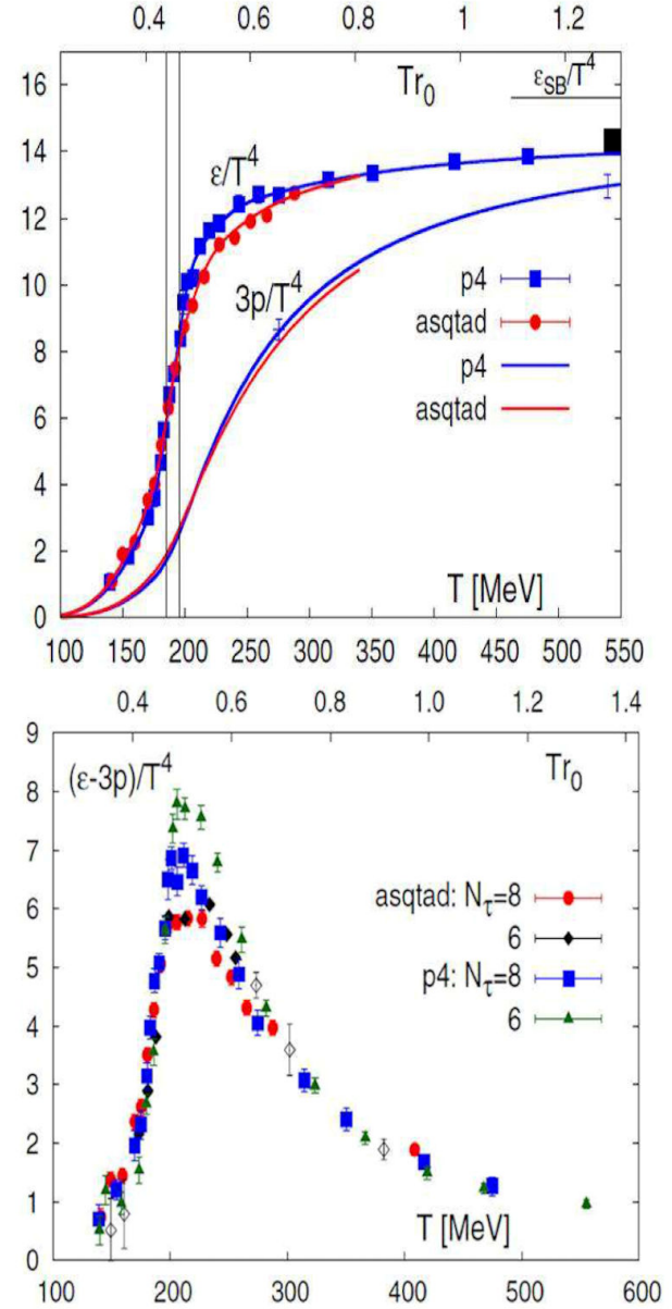
FIGURE 2. The energy density and the pressure as the function of temperature (up). The energy density shows a sharp rise in the temperature region 170-200 MeV. The interaction measure calculated using different staggered fermion actions (bottom) [58].
