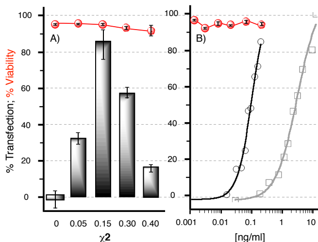
Figure 3. A) Transfection efficiency (grey bars) and cell viability (red circles) in HeLa-EGFP, at a constant siRNA (14 nM) and P1(1) 85 (2) 15 (4 \mu\text{M} ) concentrations and prepared with different molar fractions of 2 . B) Dose-response curves of lead candidate P1(1) 85 (2) 15 (black circles, EC_{50} = 0.09 \text{ ng/mL} ) and Lipofectamine RNAiMAX ® (grey squares, EC_{50} = 2.5 \text{ ng/mL} ) and cell viability for P1(1) 85 (2) 15 (red circles).
