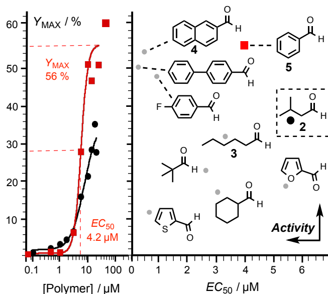
Figure 2. Representation of Y_{\text{max}} vs EC_{50} for the DNA transport experiments in EYPC-LUVs \Delta HPTS/DPX for hydrazone-activated polymers at \chi_{\text{Hydrophobic}} : 0.15 and \chi_1 : 0.85.
