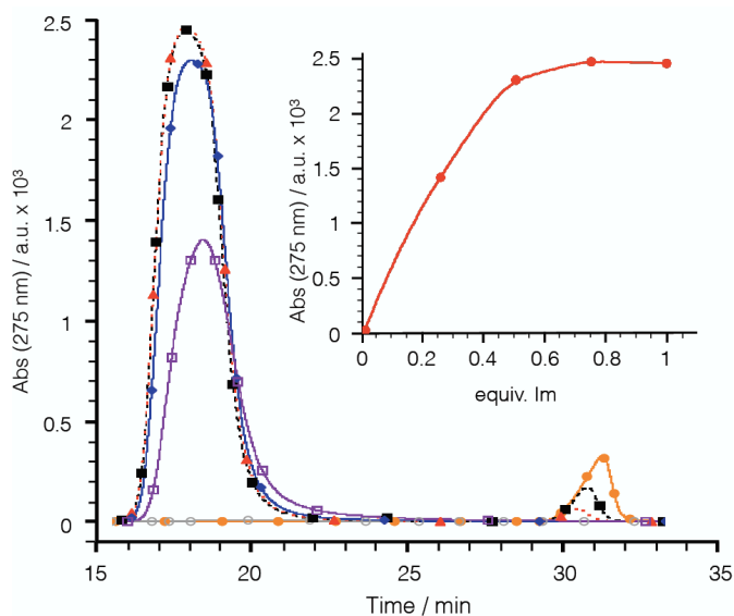
Figure 1. GPC ( \lambda_{\text{Abs}} = 275 \text{ nm} ) analysis of P1 incubated with (1 (■), 0.75 (▲), 0.5 (◆), 0.25 (□), 0 (○) equiv and pure (●) 4-imidazolecarboxaldehyde; Conditions: (100 mM acetic acid, pH 2.9, 2 h). Inset: Increase in absorbance of the high molecular weight peak ( R_t 18 min) with increasing amounts of 4-imidazolecarboxaldehyde.
